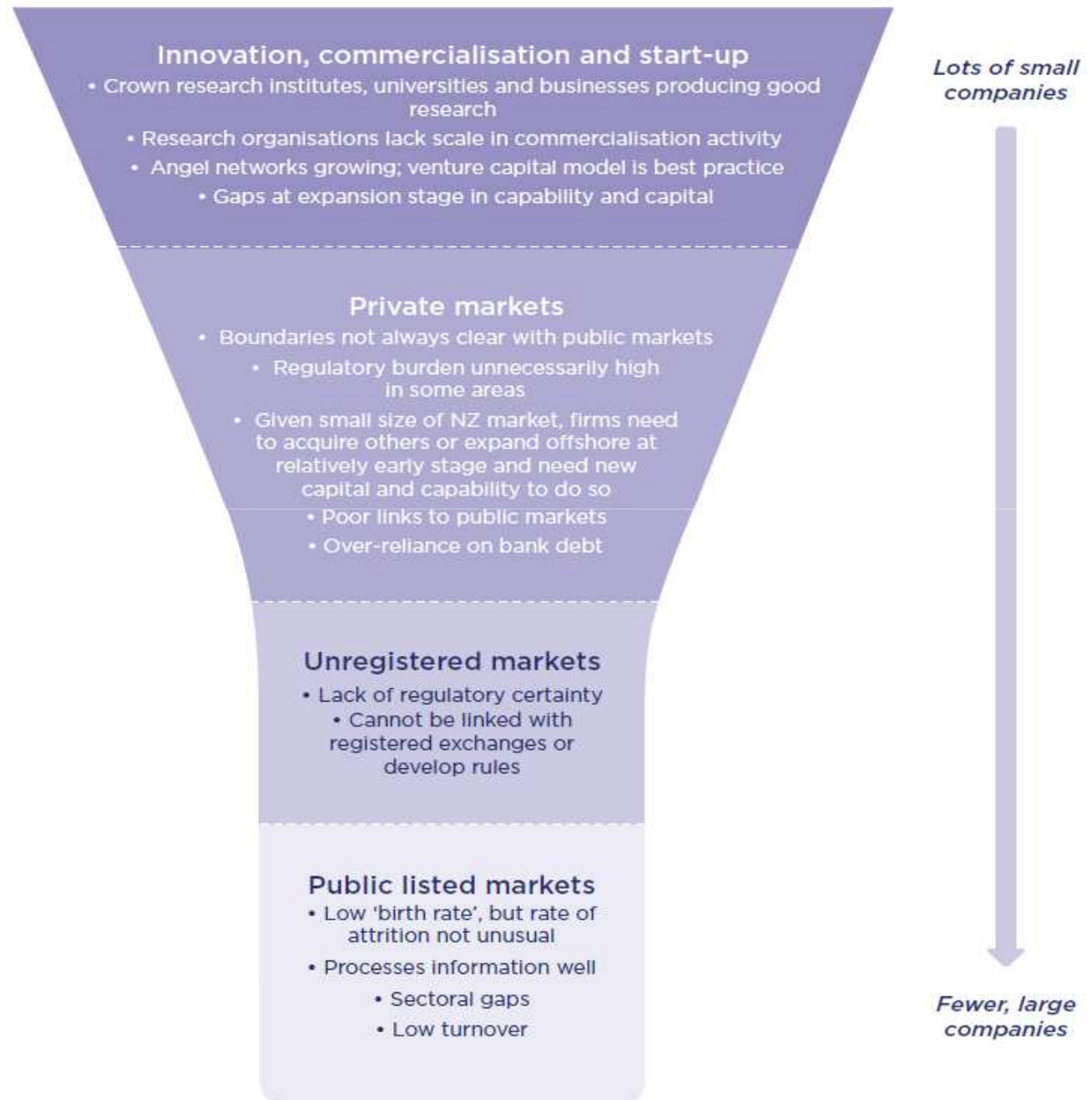
Figure 3. Equity market observations
